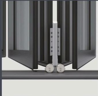
High-low track design Good water tightness
