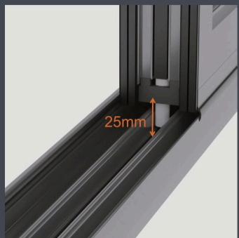
Top and bottom shoot bolts Adds strength, resists super typhoons
